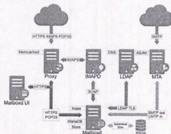
Picture 1- Zimbra single-server architecture
